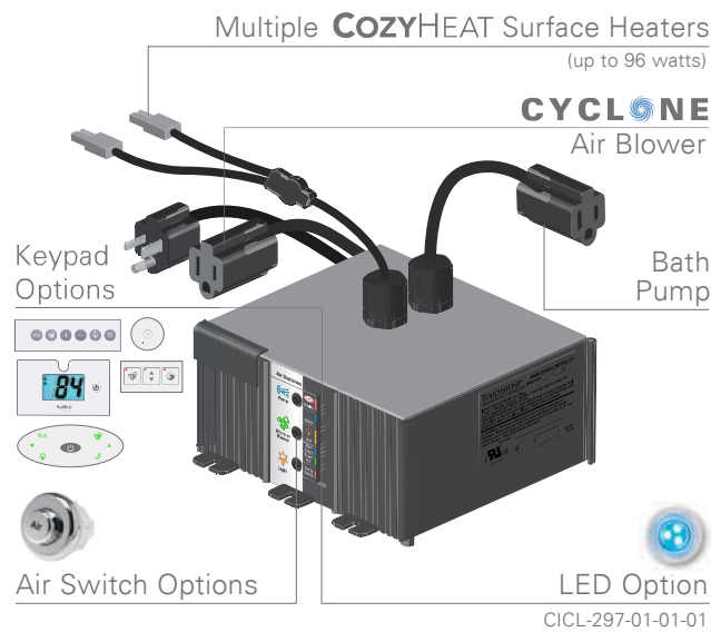
CMBC-298 Series MASTER BATH CONTROLLER Water & Air Massage System with CozyHeat Option
