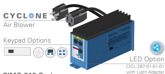
CIMC-213 Series COMMAND AIR, COMMAND AIR PLUS Air Massage System with Electronic Keypad Option
